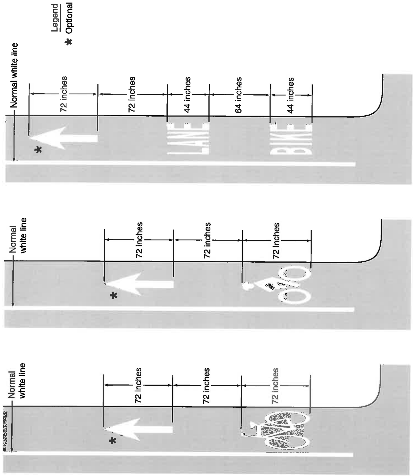
Figure 9C-3. Word, Symbol, and Arrow Pavement Markings for Bicycle Lanes
